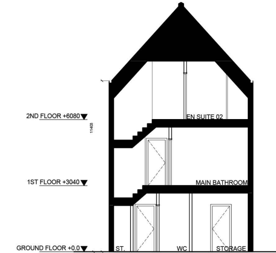
Typical Townhouse Section
