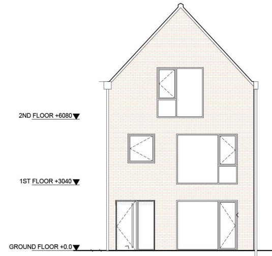
Typical Townhouse Elevation
