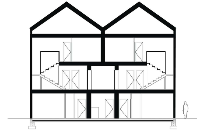
Typical Duplex Section
