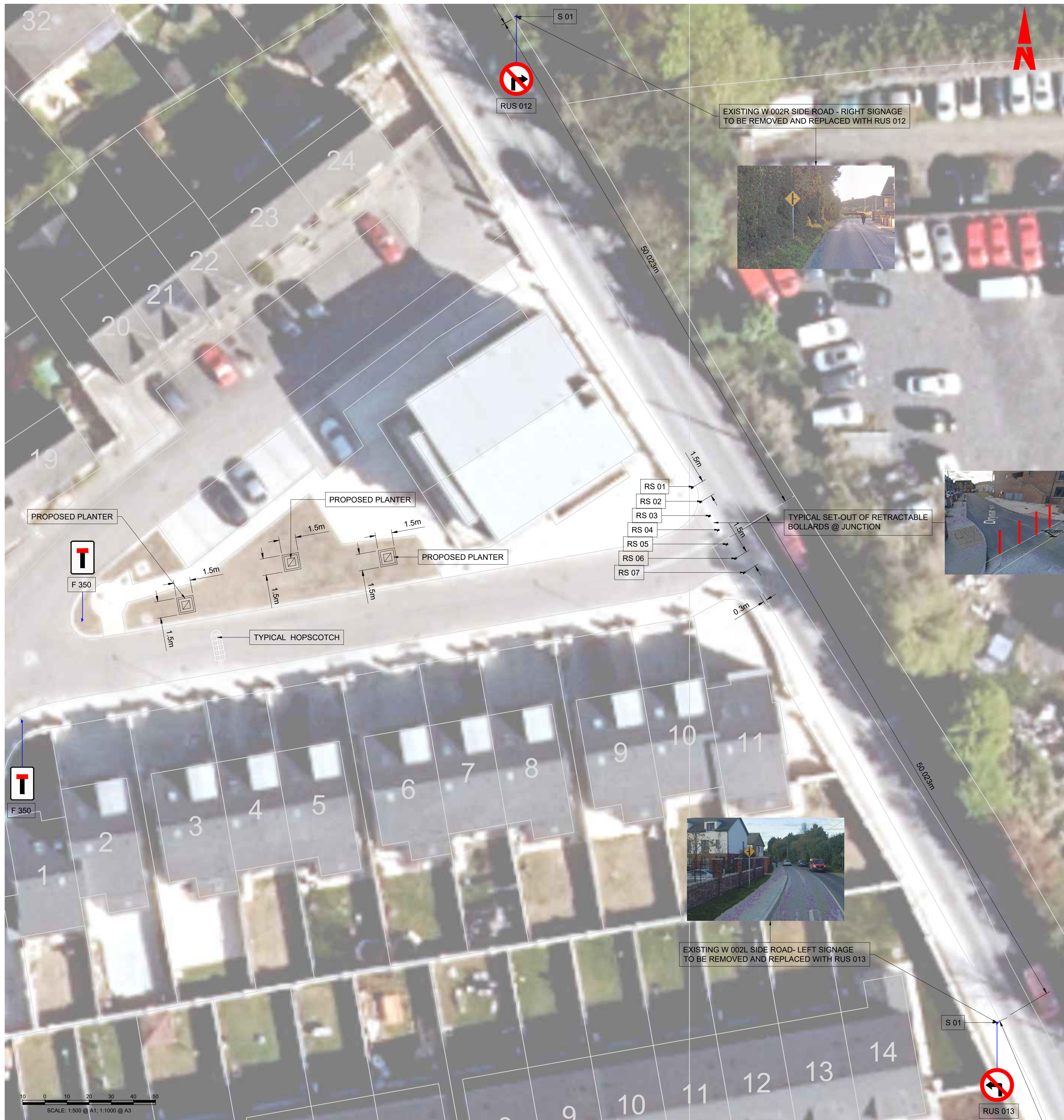
DRYNAM HEATH QUIET STREETS - OPTION 3 Scale 1:200
