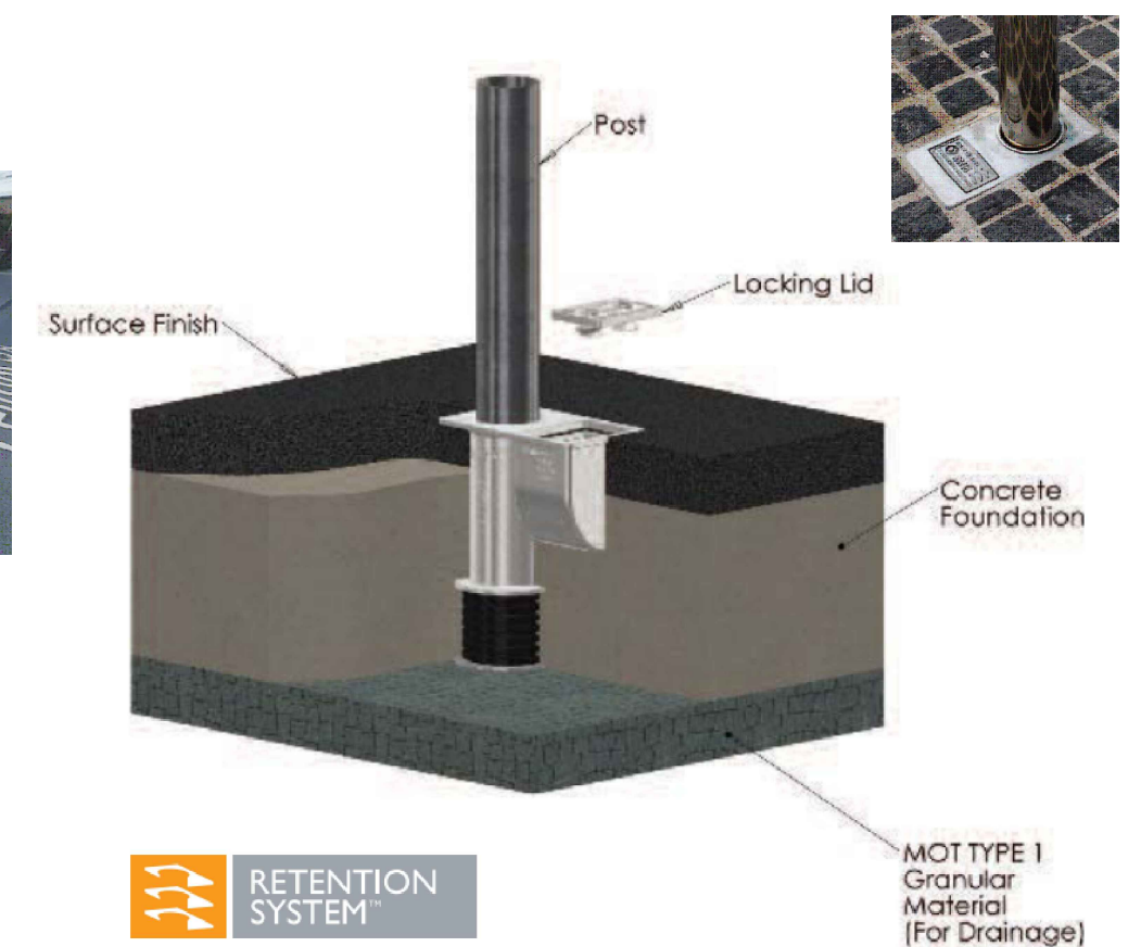
TYPICAL RETENTION SYSTEM Scale: nts
